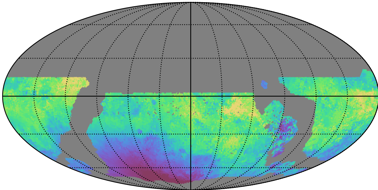
weather_cloudso1v3.4_10yrs WFD u band: Median moonDistance
