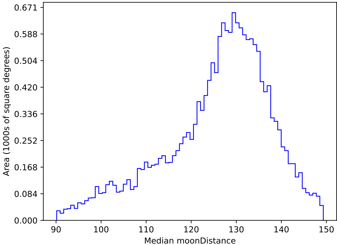
weather_cloudso1v3.4_10yrs WFD u band: Median moonDistance
