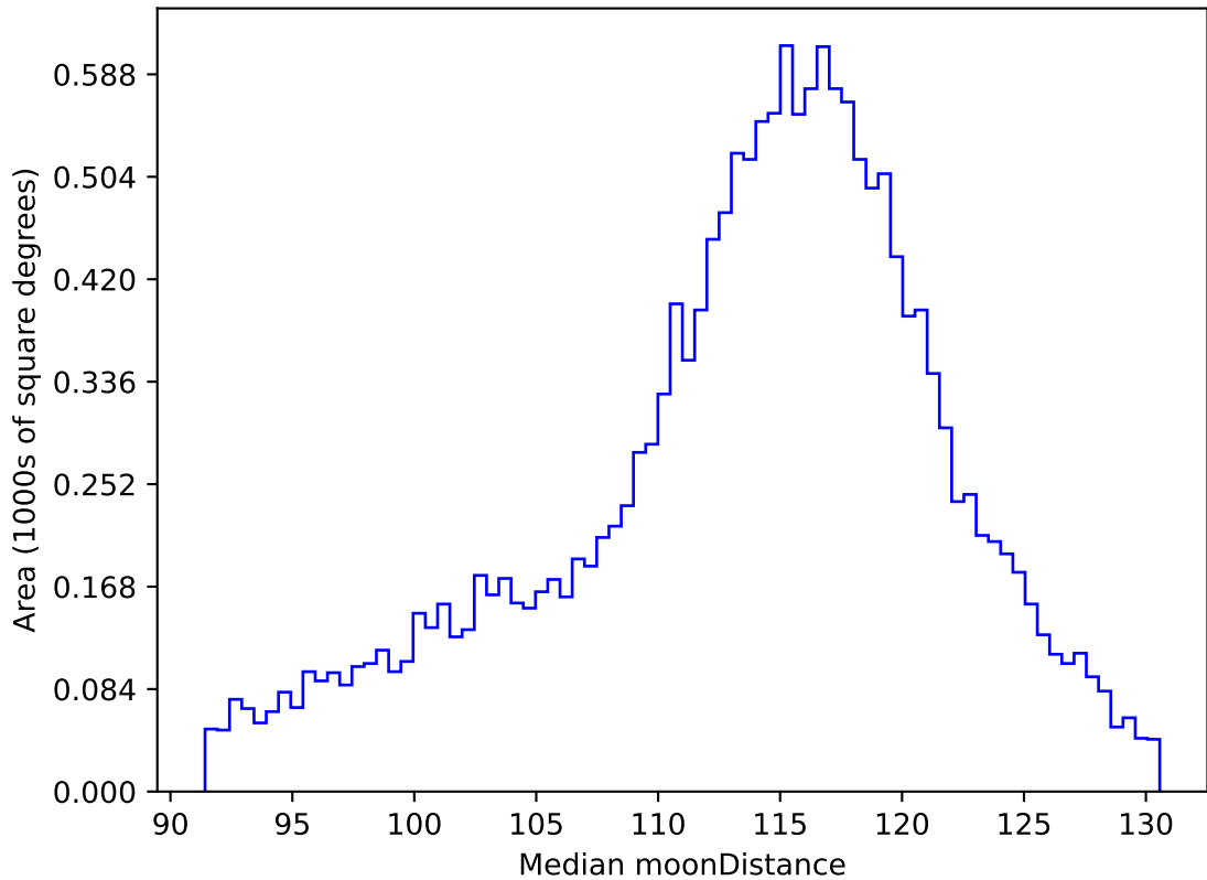
weather_cloudso1v3.4_10yrs WFD r band: Median moonDistance
