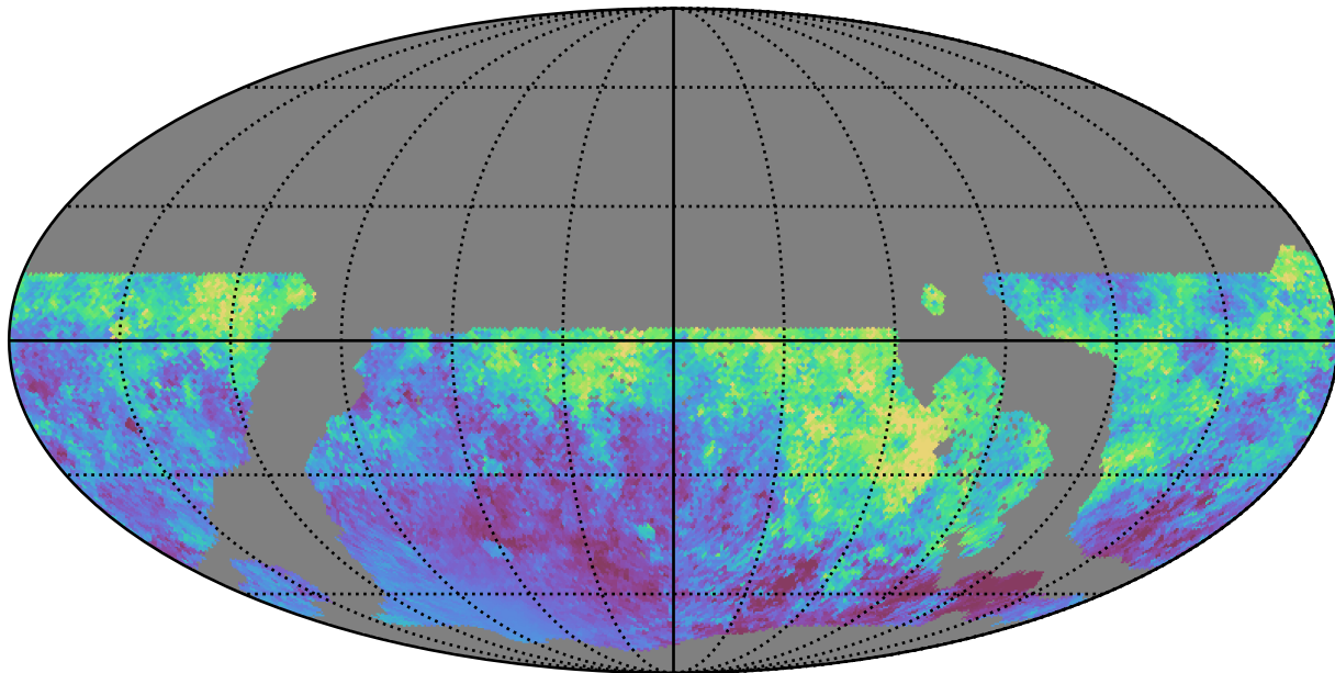
weather_cloudso1v3.4_10yrs WFD i band: Median moonDistance
