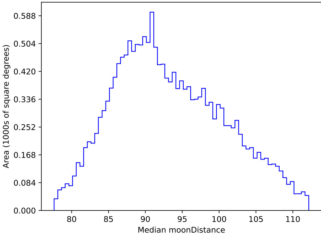
weather_cloudso1v3.4_10yrs WFD i band: Median moonDistance
