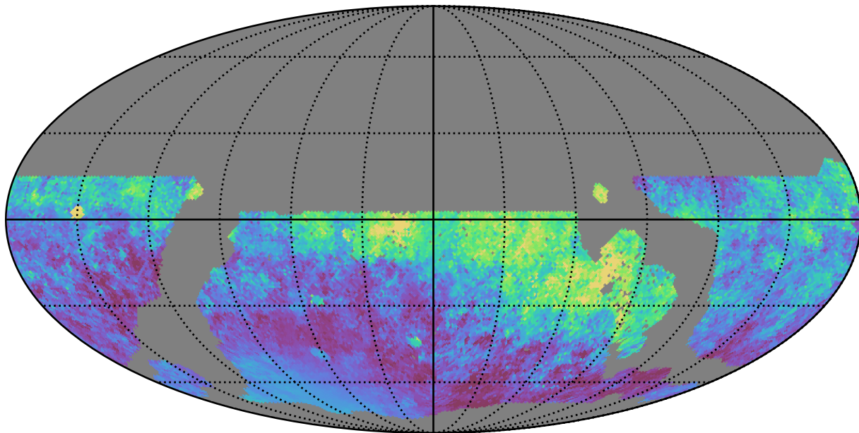
weather_cloudso1v3.4_10yrs WFD all bands: Median moonDistance
