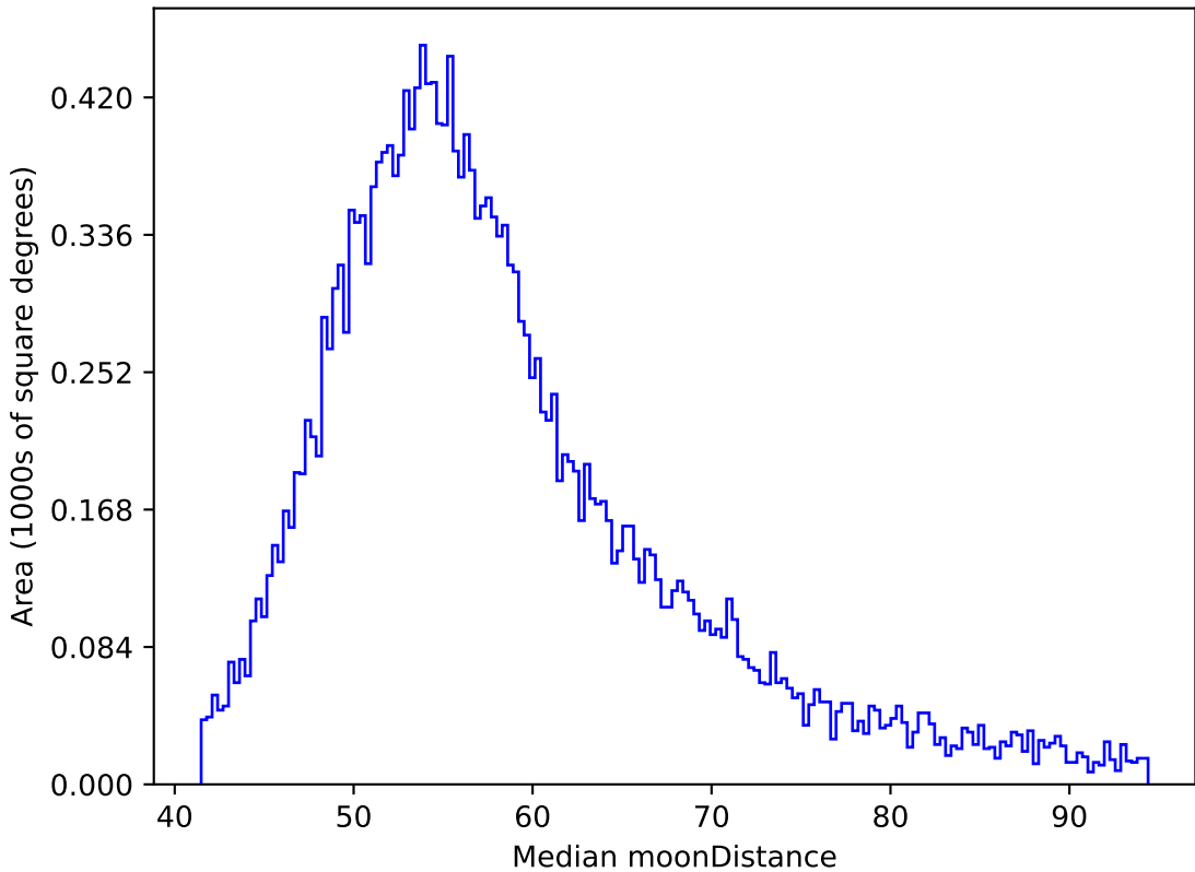
weather_cloudso1v3.4_10yrs All sky y band: Median moonDistance
