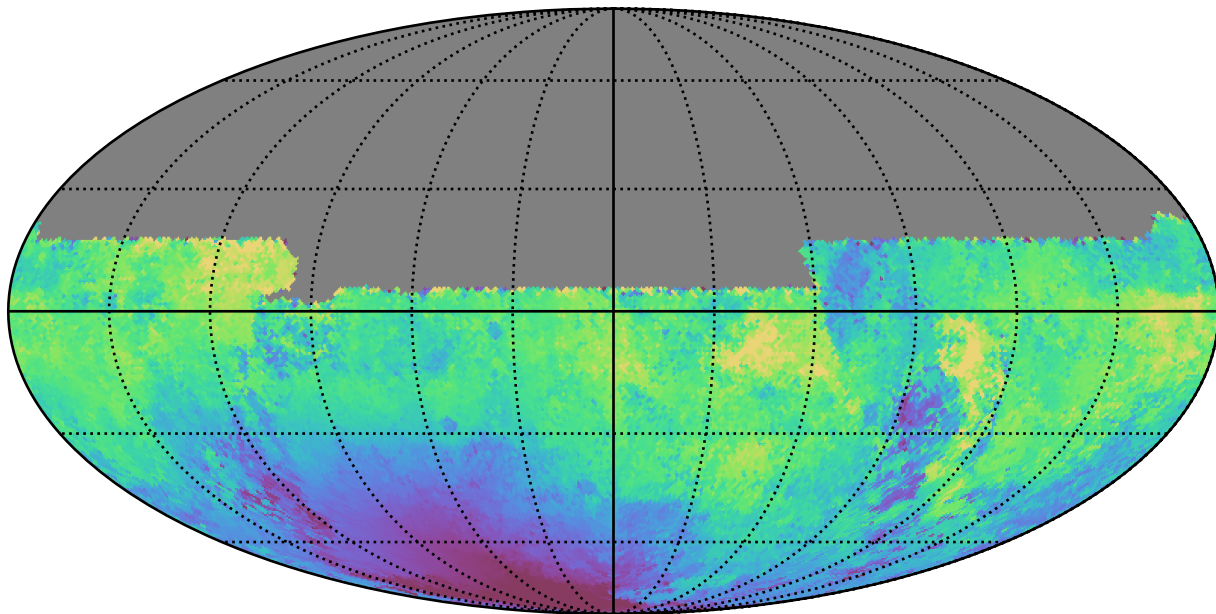
weather_cloudso1v3.4_10yrs All sky u band: Median moonDistance
