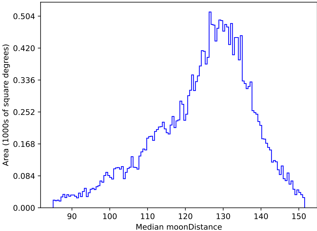
weather_cloudso1v3.4_10yrs All sky u band: Median moonDistance
