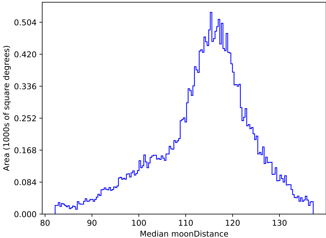
weather_cloudso1v3.4_10yrs All sky r band: Median moonDistance
