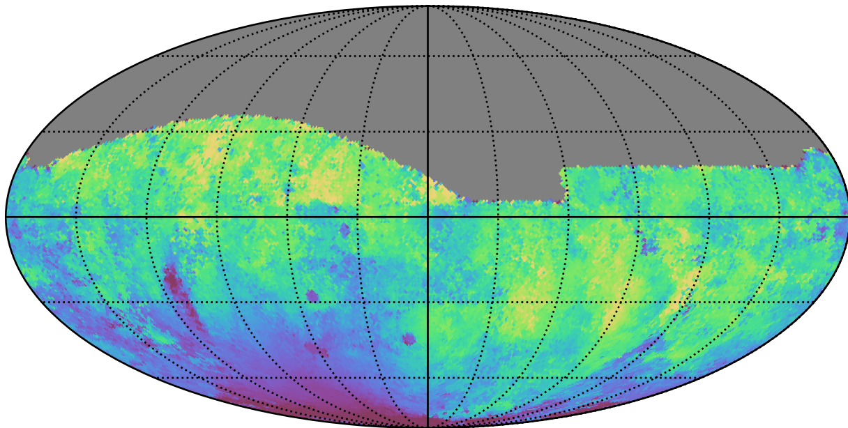
weather_cloudso1v3.4_10yrs All sky g band: Median moonDistance
