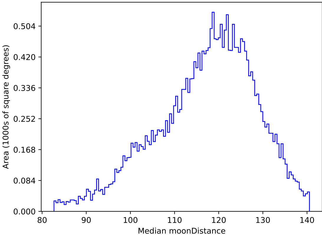
weather_cloudso1v3.4_10yrs All sky g band: Median moonDistance
