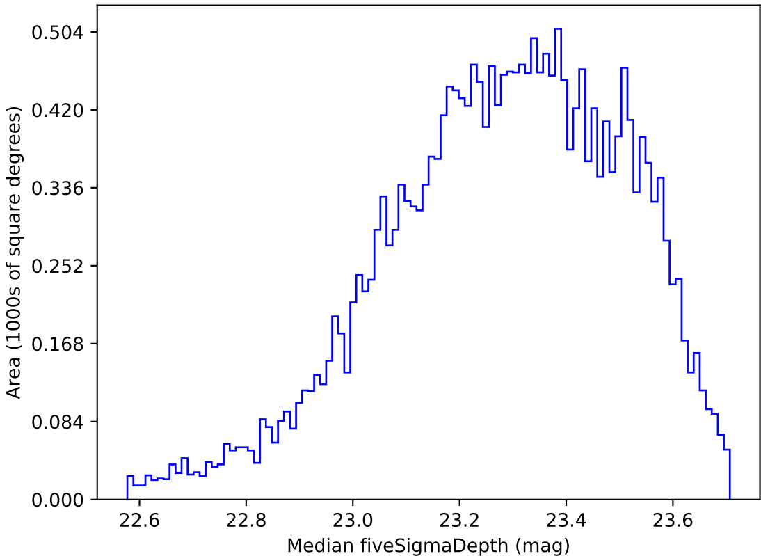
weather_cloudso1v3.4_10yrs Yr 1 u band: Median fiveSigmaDepth
