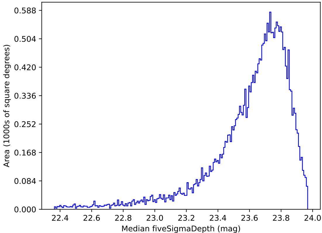
weather_cloudso1v3.4_10yrs Yr 1 i band: Median fiveSigmaDepth
