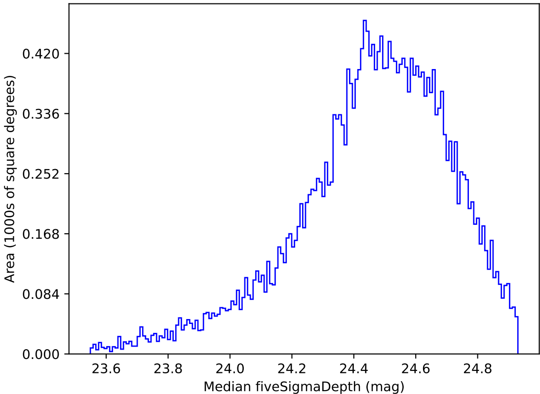
weather_cloudso1v3.4_10yrs Yr 1 g band: Median fiveSigmaDepth
