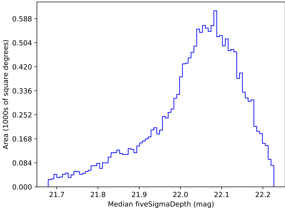
weather_cloudso1v3.4_10yrs WFD y band: Median fiveSigmaDepth
