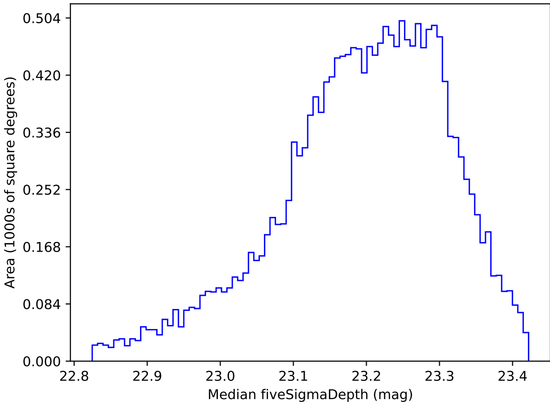
weather_cloudso1v3.4_10yrs WFD u band: Median fiveSigmaDepth
