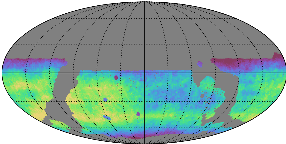
weather_cloudso1v3.4_10yrs WFD r band: Median fiveSigmaDepth
