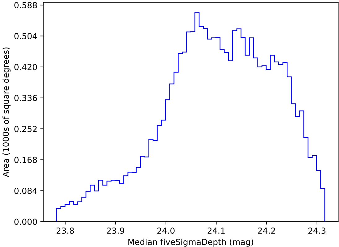
weather_cloudso1v3.4_10yrs WFD r band: Median fiveSigmaDepth
