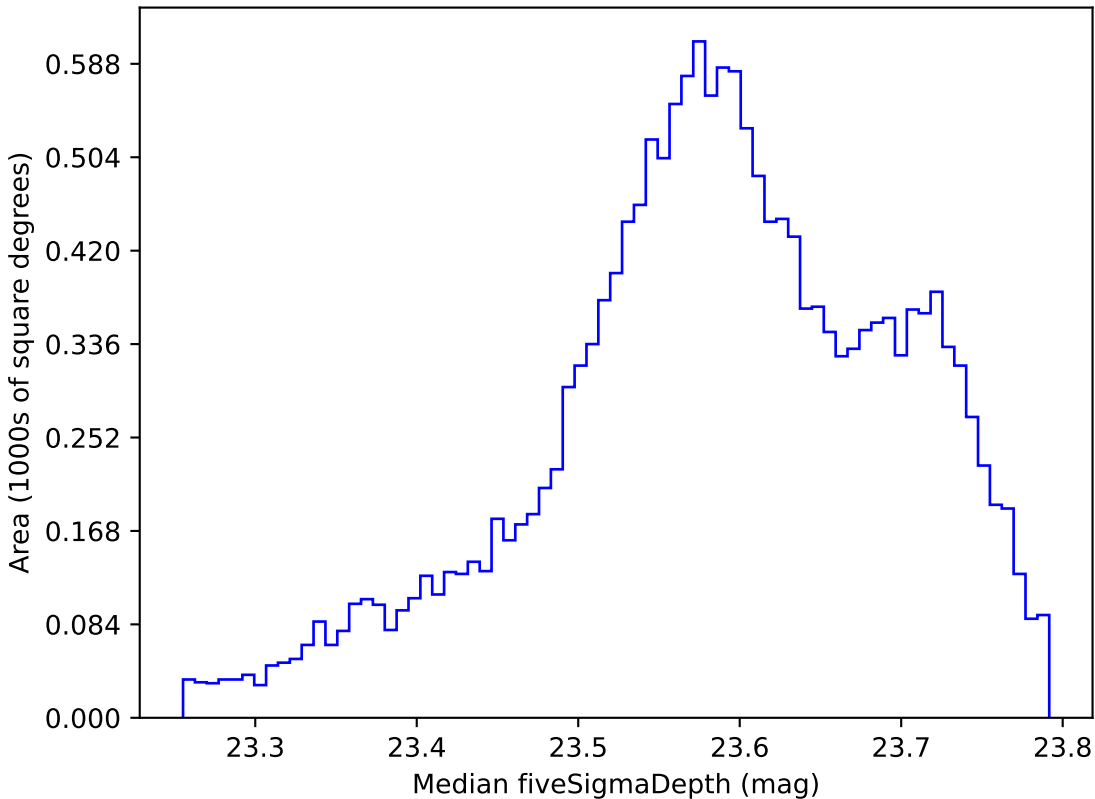
weather_cloudso1v3.4_10yrs WFD i band: Median fiveSigmaDepth
