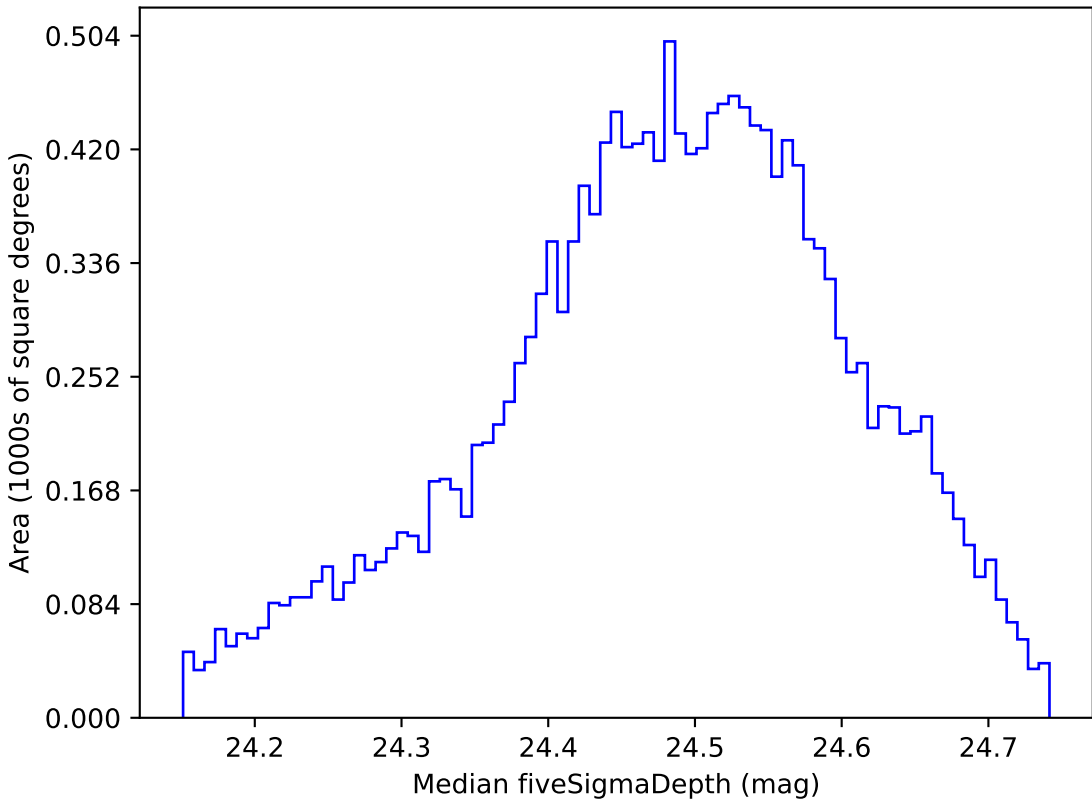
weather_cloudso1v3.4_10yrs WFD g band: Median fiveSigmaDepth
