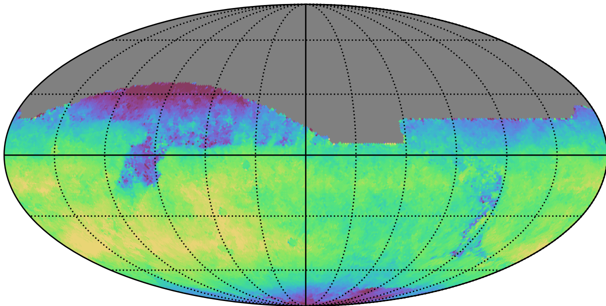
weather_cloudso1v3.4_10yrs All sky z band: Median fiveSigmaDepth
