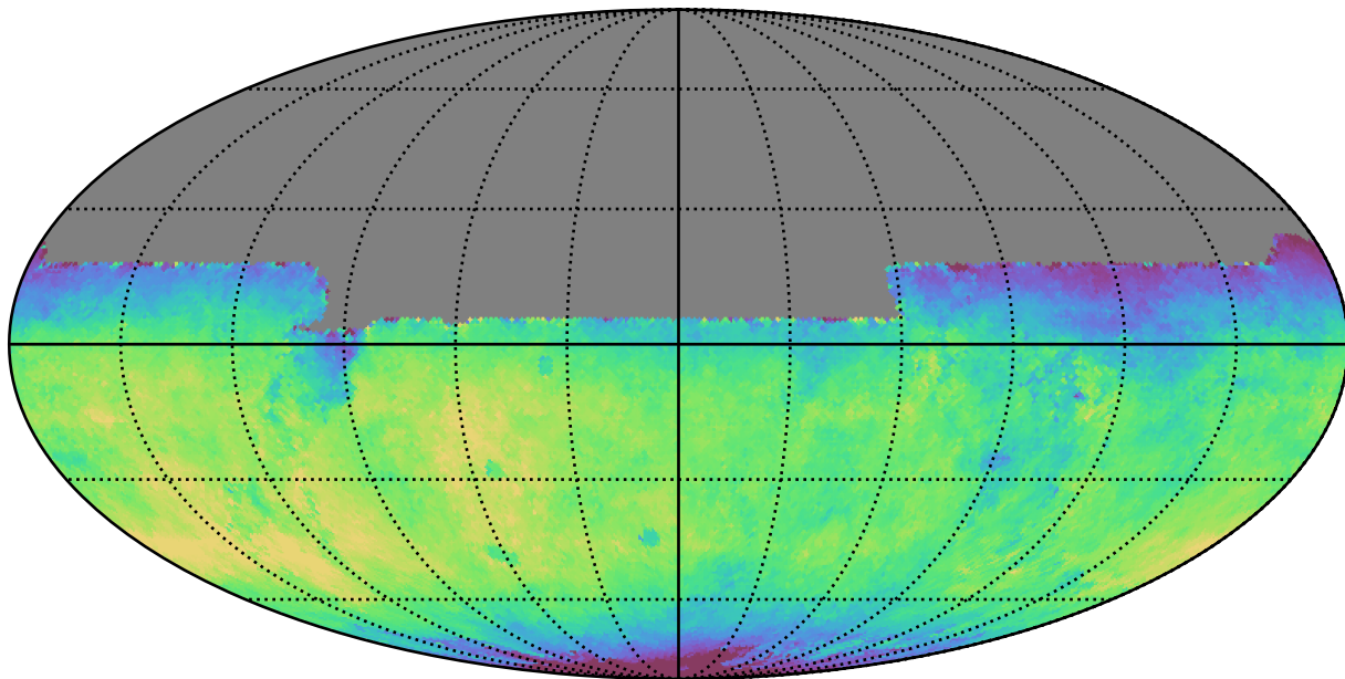
weather_cloudso1v3.4_10yrs All sky y band: Median fiveSigmaDepth
