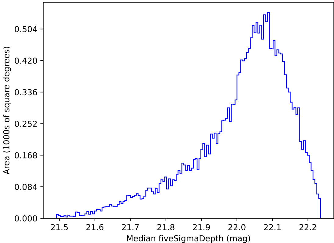
weather_cloudso1v3.4_10yrs All sky y band: Median fiveSigmaDepth
