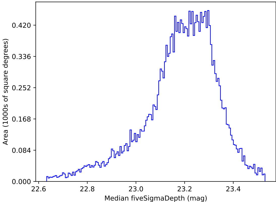
weather_cloudso1v3.4_10yrs All sky u band: Median fiveSigmaDepth
