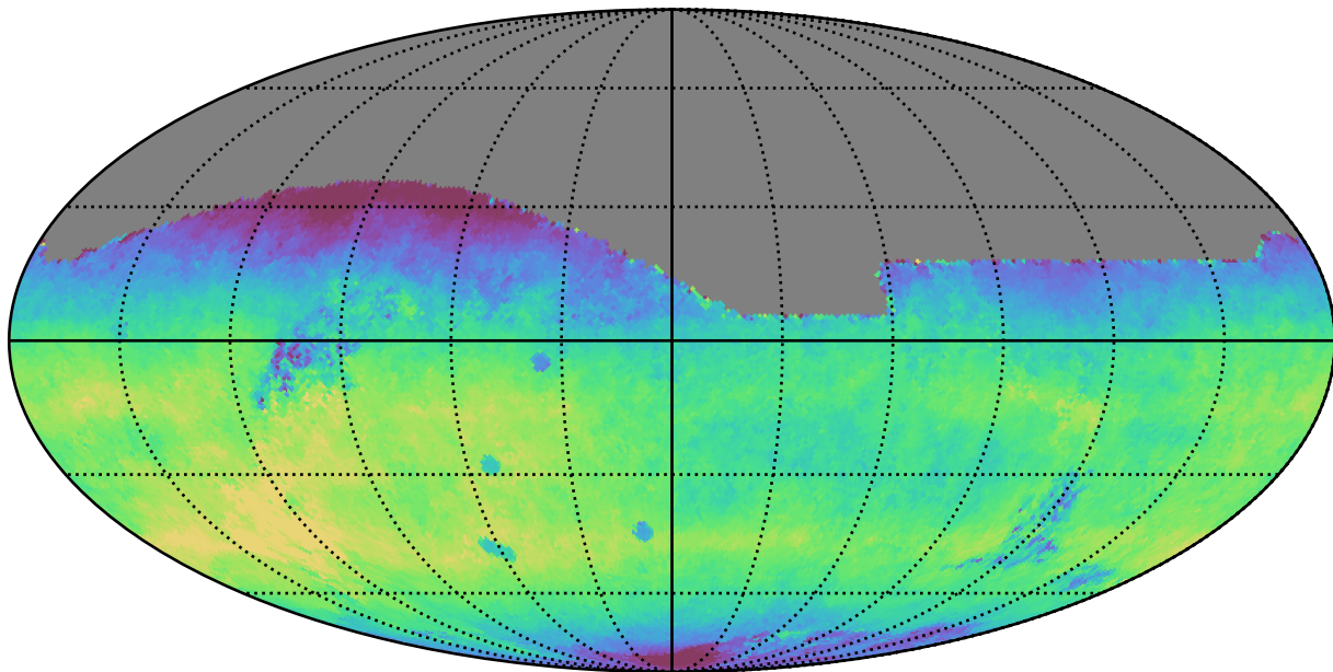
weather_cloudso1v3.4_10yrs All sky r band: Median fiveSigmaDepth
