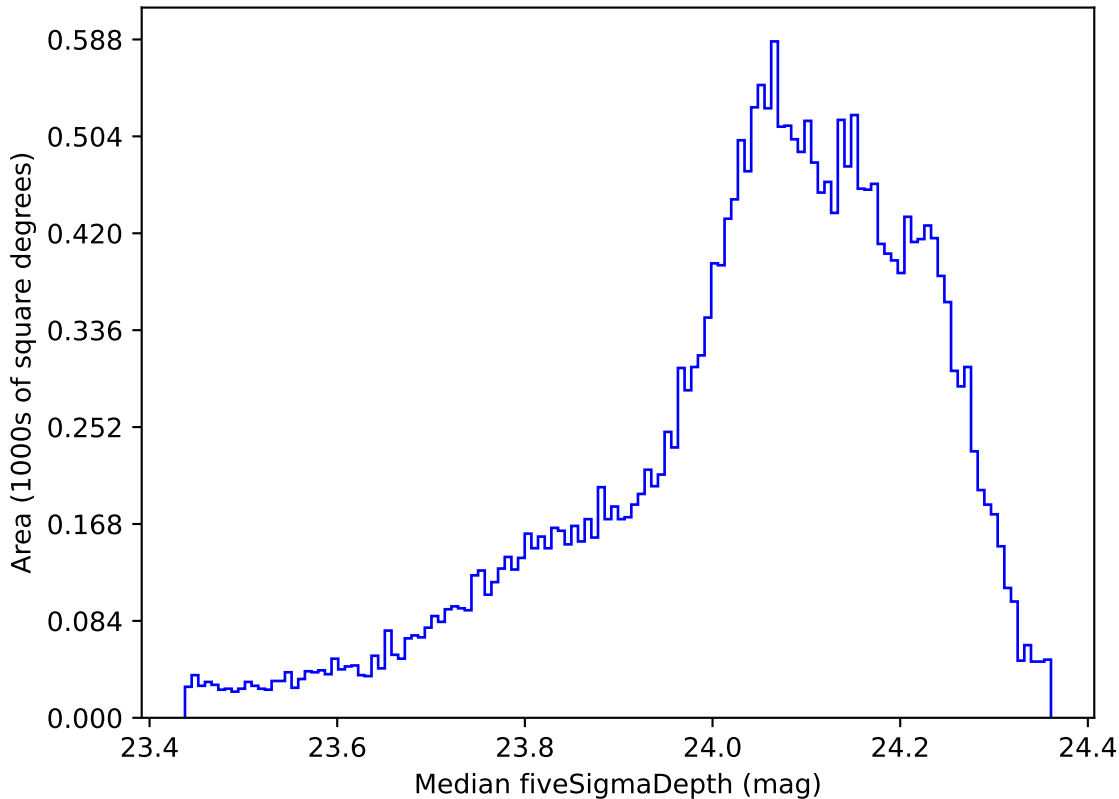
weather_cloudso1v3.4_10yrs All sky r band: Median fiveSigmaDepth
