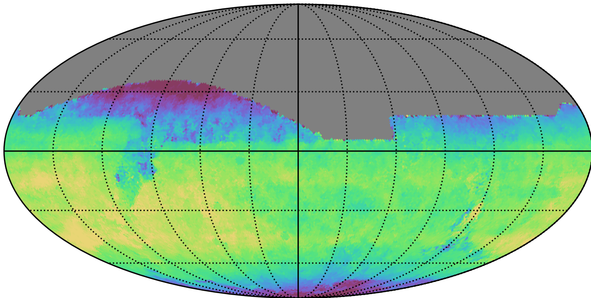
weather_cloudso1v3.4_10yrs All sky i band: Median fiveSigmaDepth
