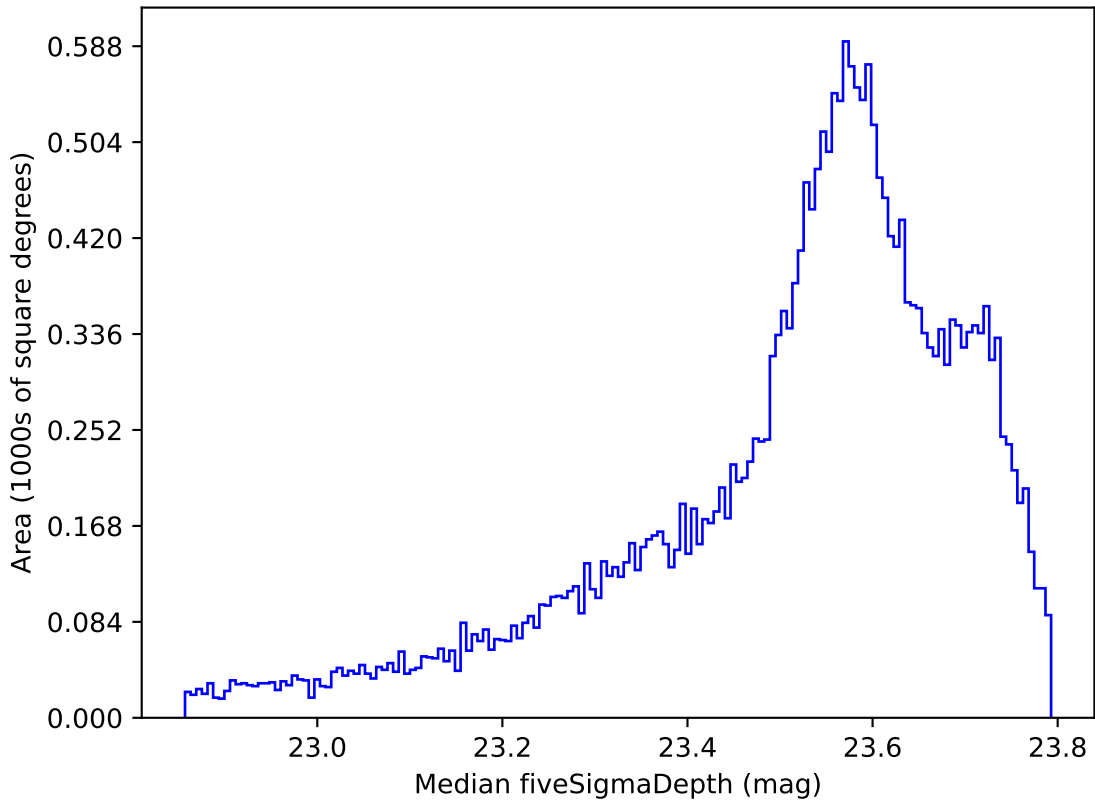
weather_cloudso1v3.4_10yrs All sky i band: Median fiveSigmaDepth
