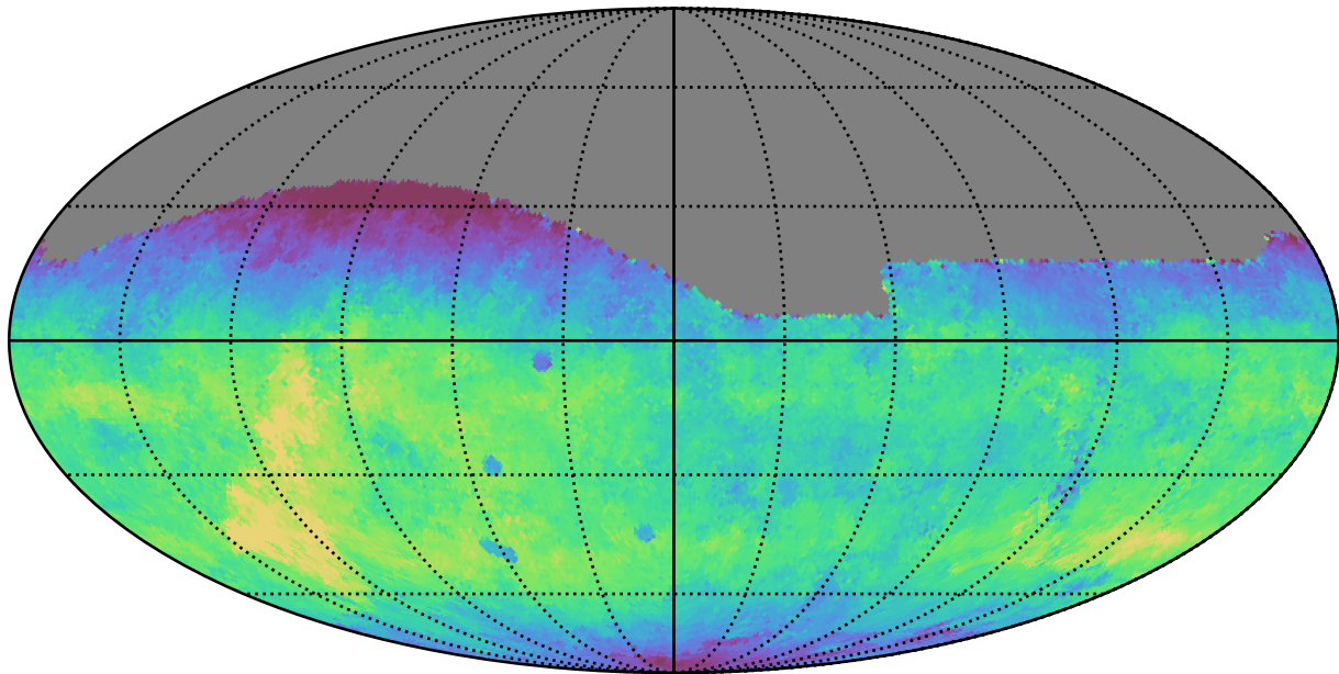
weather_cloudso1v3.4_10yrs All sky g band: Median fiveSigmaDepth
