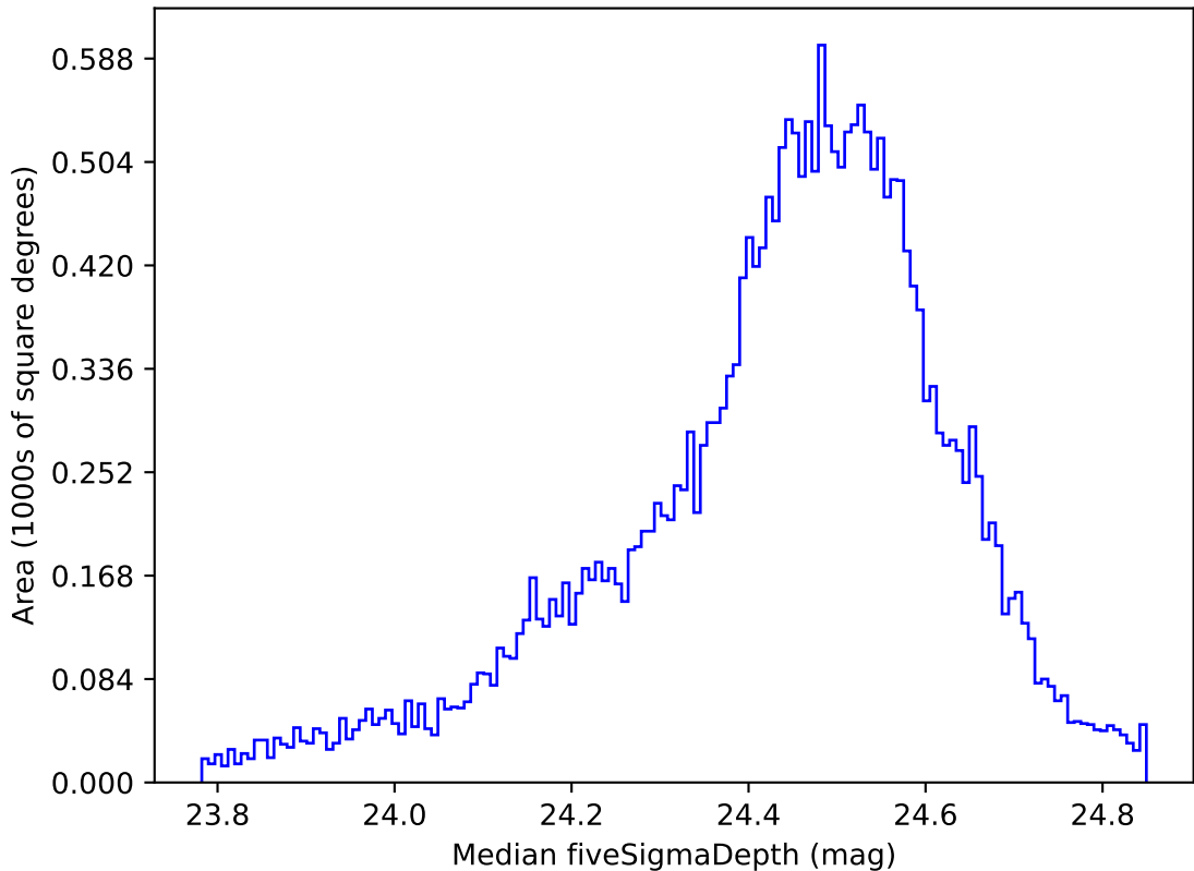
weather_cloudso1v3.4_10yrs All sky g band: Median fiveSigmaDepth
