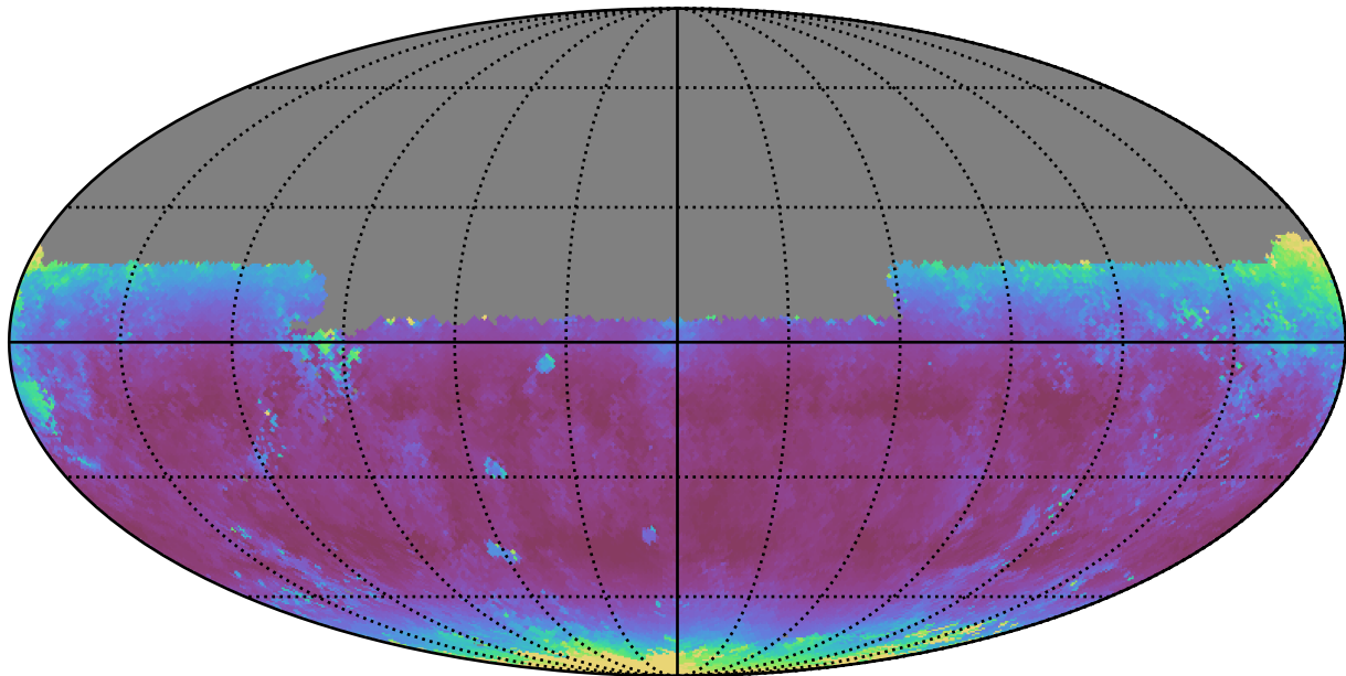
weather_cloudso1v3.4_10yrs Yr 1 y band: Median airmass
