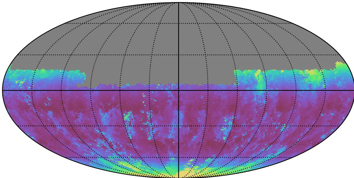
weather_cloudso1v3.4_10yrs Yr 1 u band: Median airmass
