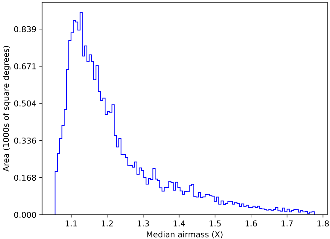
weather_cloudso1v3.4_10yrs Yr 1 u band: Median airmass
