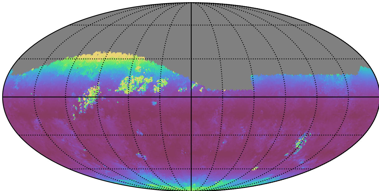
weather_cloudso1v3.4_10yrs Yr 1 r band: Median airmass
