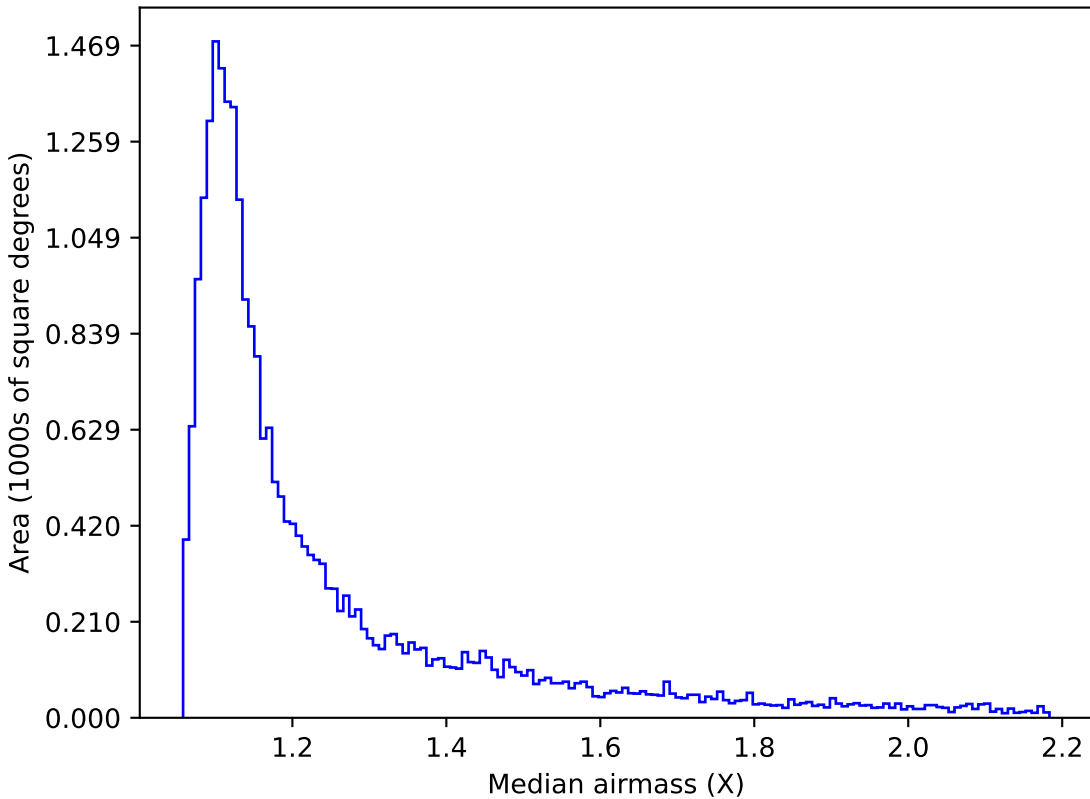
weather_cloudso1v3.4_10yrs Yr 1 r band: Median airmass
