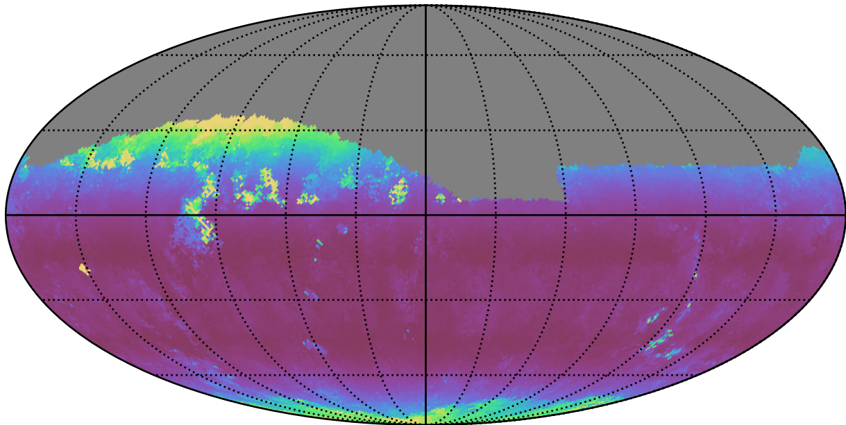
weather_cloudso1v3.4_10yrs Yr 1 i band: Median airmass
