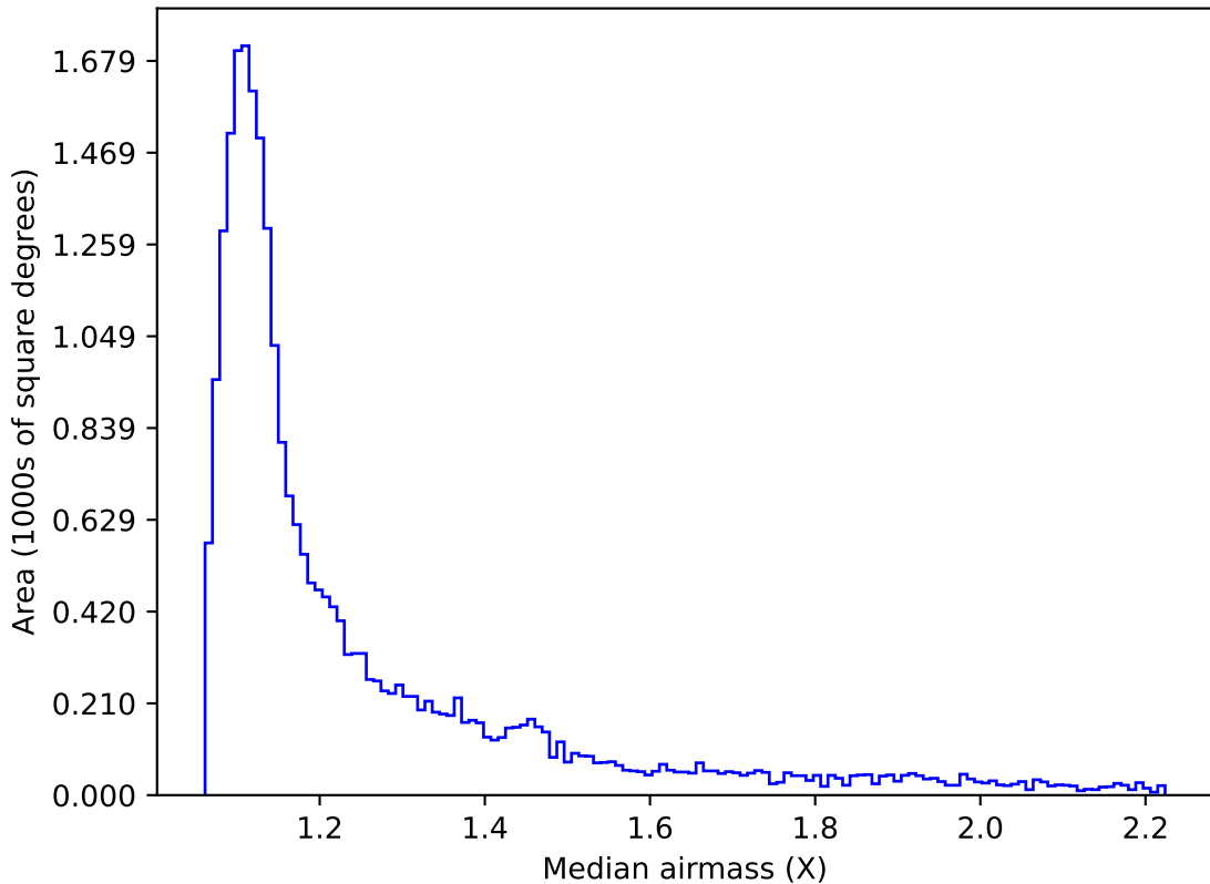
weather_cloudso1v3.4_10yrs Yr 1 i band: Median airmass
