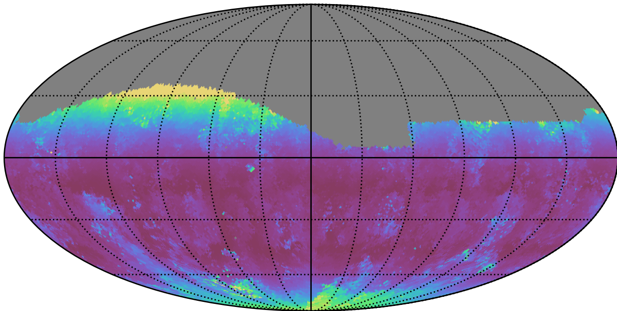
weather_cloudso1v3.4_10yrs Yr 1 g band: Median airmass
