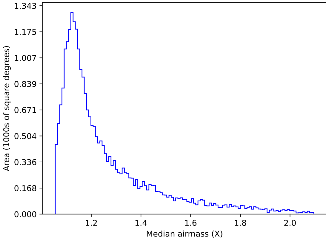
weather_cloudso1v3.4_10yrs Yr 1 g band: Median airmass
