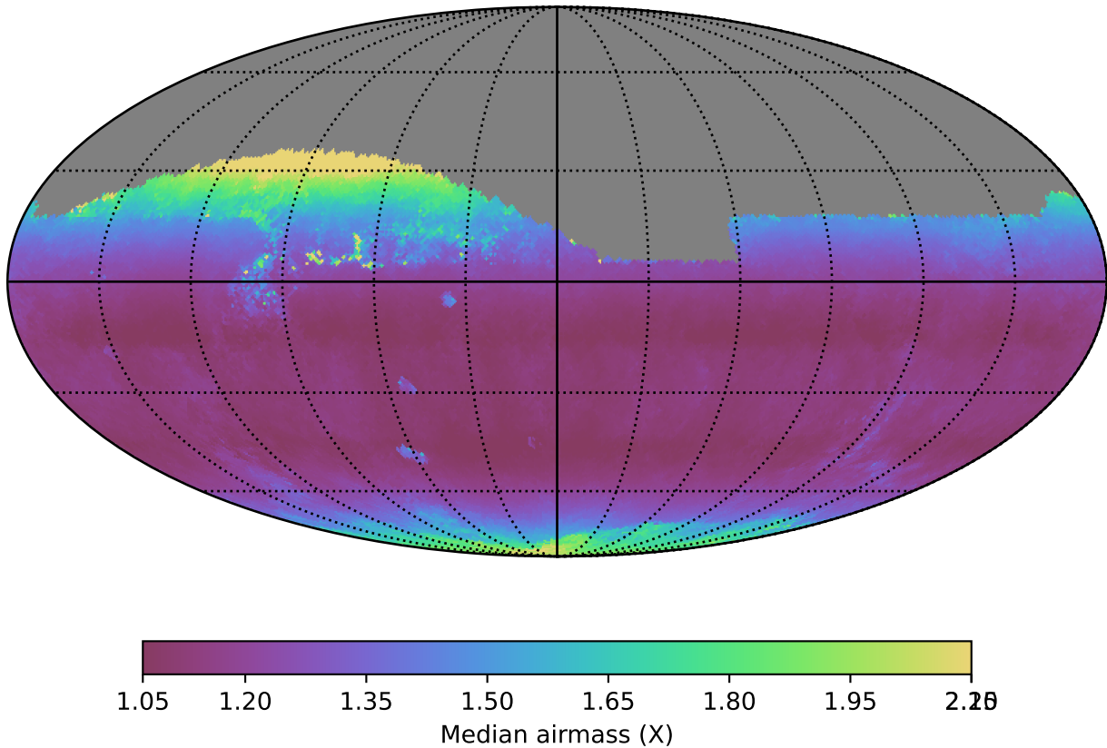
weather_cloudso1v3.4_10yrs Yr 1 all bands: Median airmass
