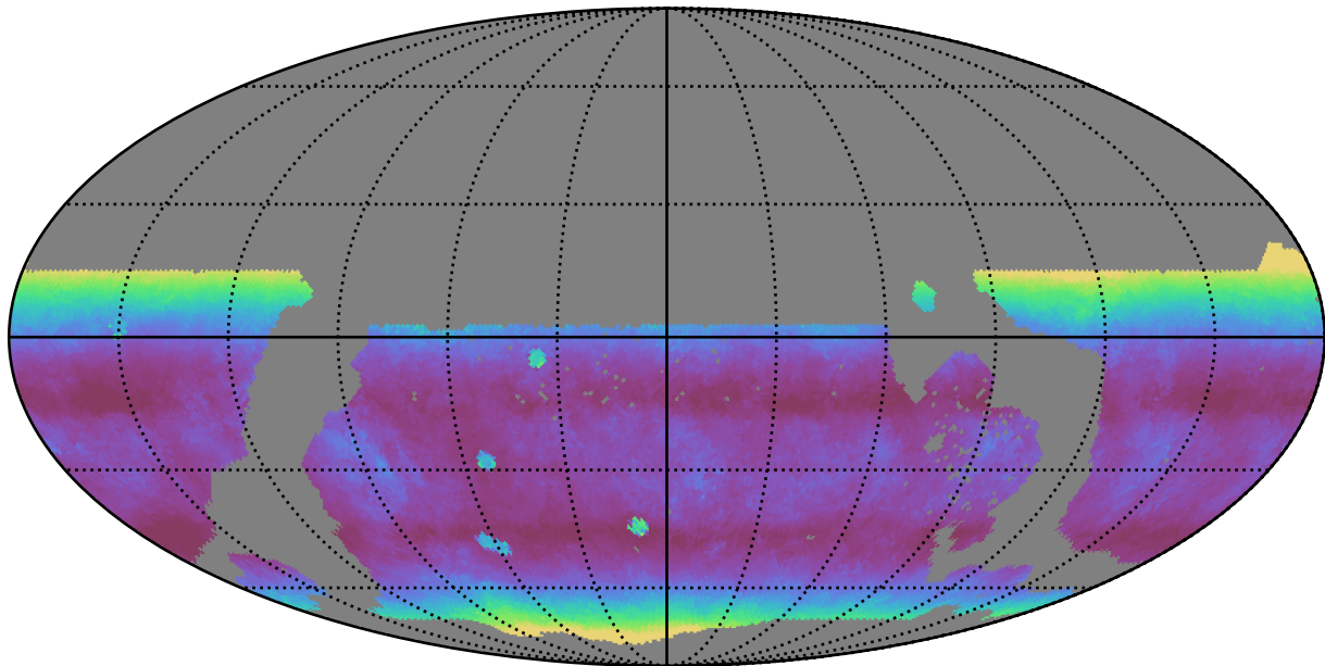
weather_cloudso1v3.4_10yrs WFD z band: Median airmass
