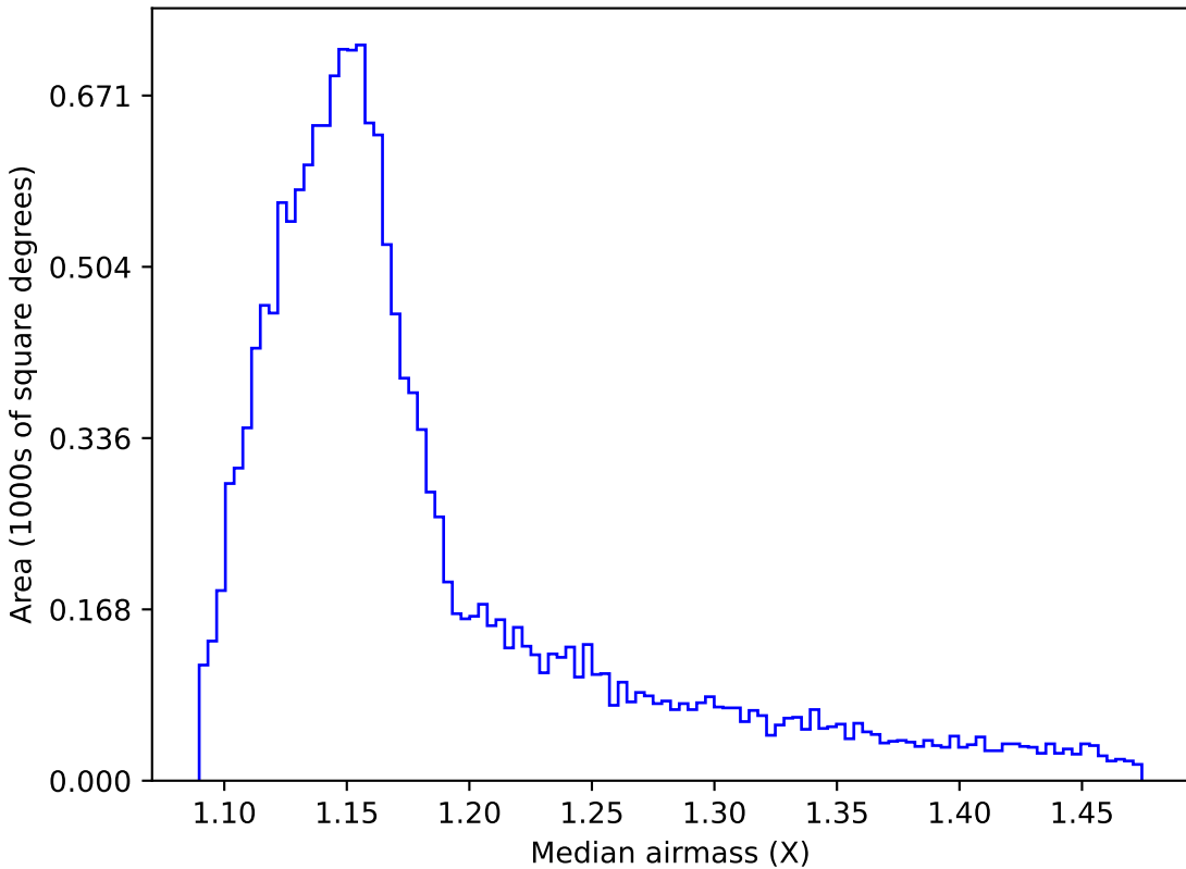
weather_cloudso1v3.4_10yrs WFD z band: Median airmass
