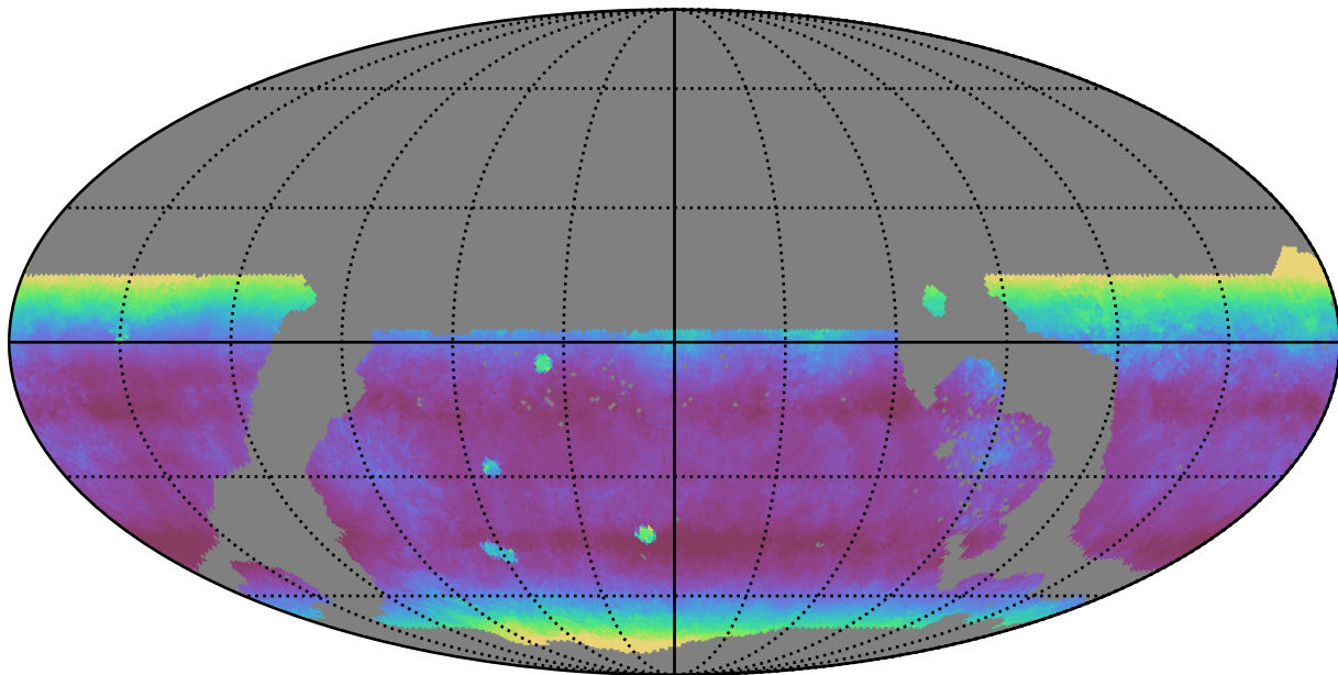
weather_cloudso1v3.4_10yrs WFD y band: Median airmass
