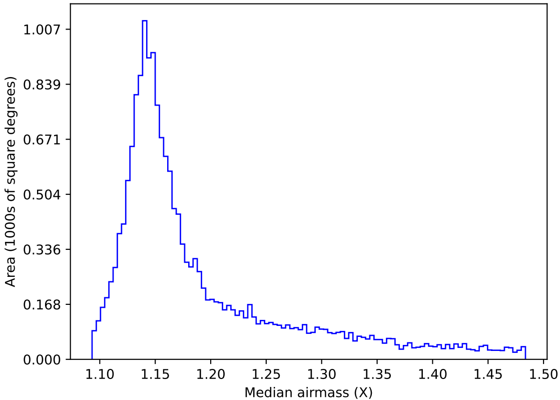
weather_cloudso1v3.4_10yrs WFD y band: Median airmass
