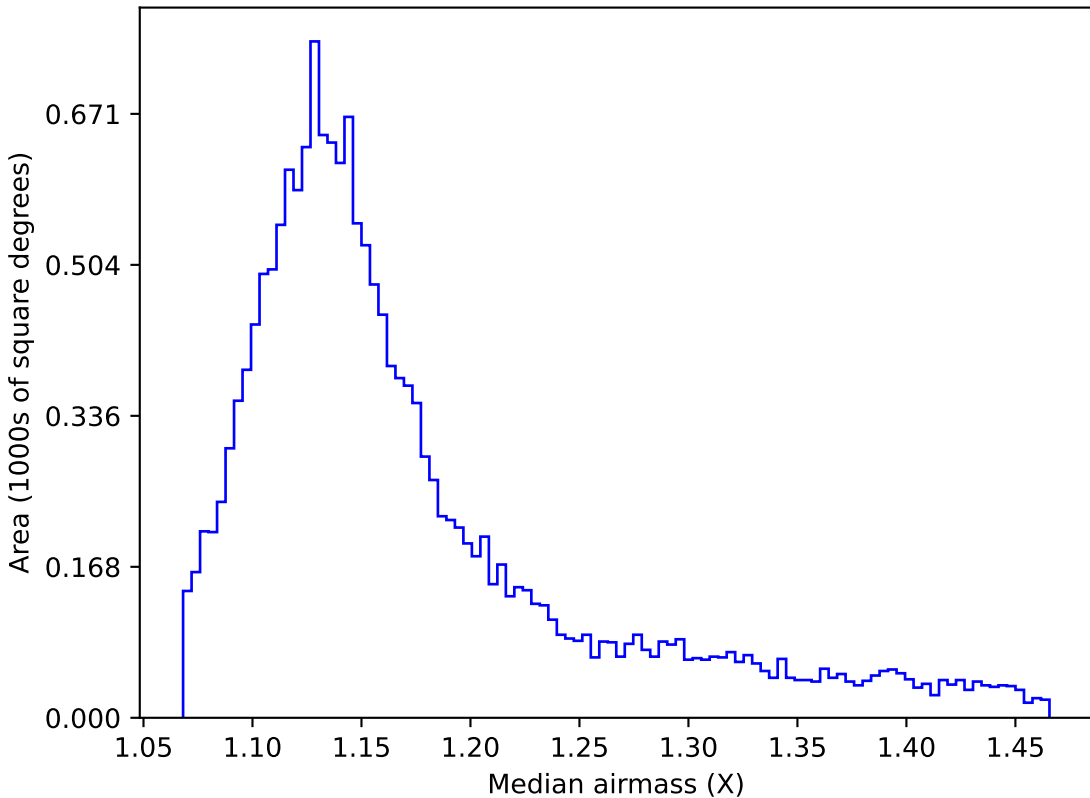
weather_cloudso1v3.4_10yrs WFD u band: Median airmass
