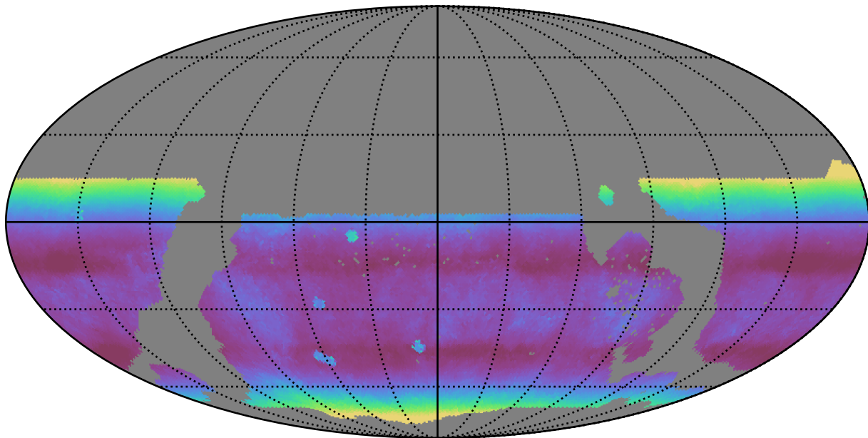
weather_cloudso1v3.4_10yrs WFD r band: Median airmass
