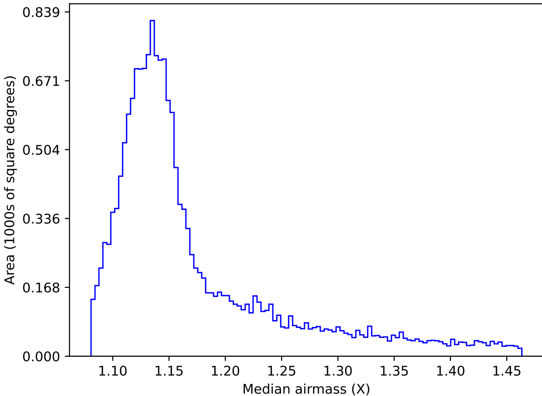
weather_cloudso1v3.4_10yrs WFD i band: Median airmass
