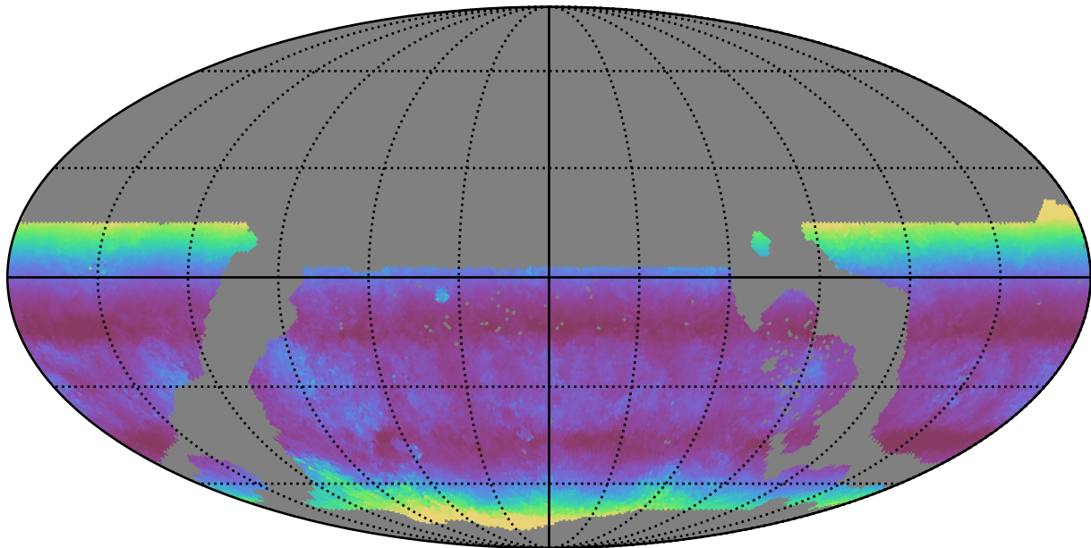
weather_cloudso1v3.4_10yrs WFD g band: Median airmass
