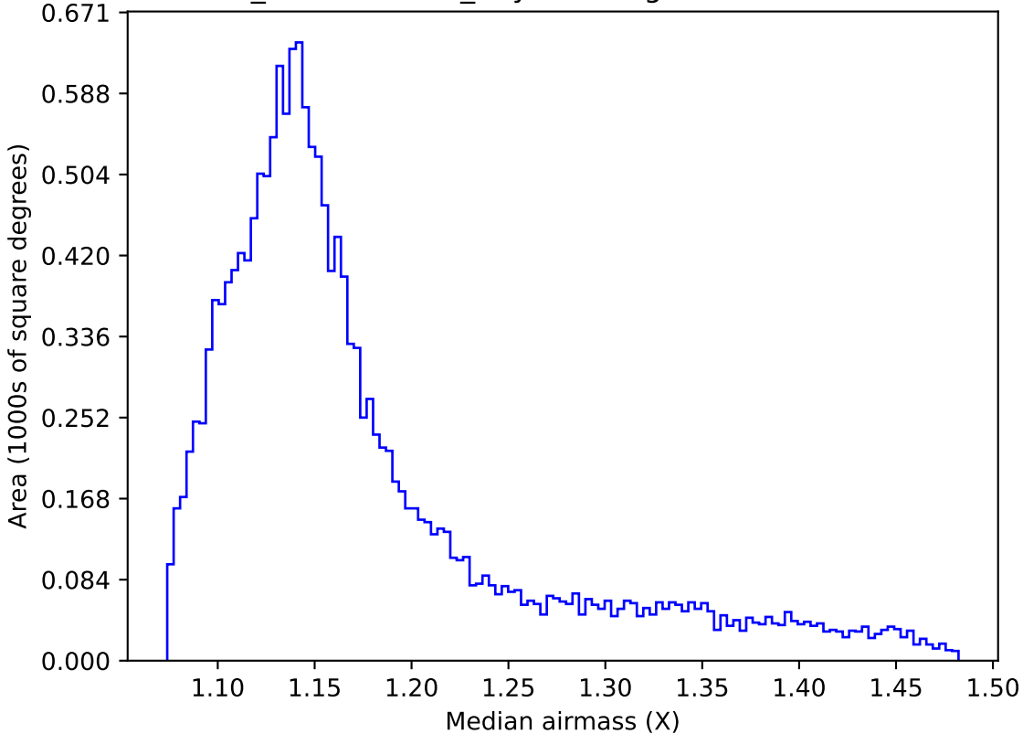
weather_cloudso1v3.4_10yrs WFD g band: Median airmass
